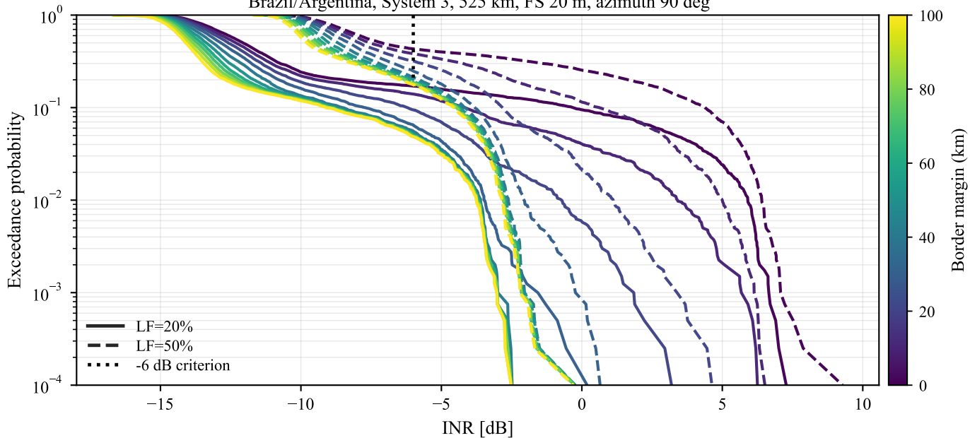
Brazil/Argentina, System 3, 525 km, FS 20 m, azimuth 90 deg
